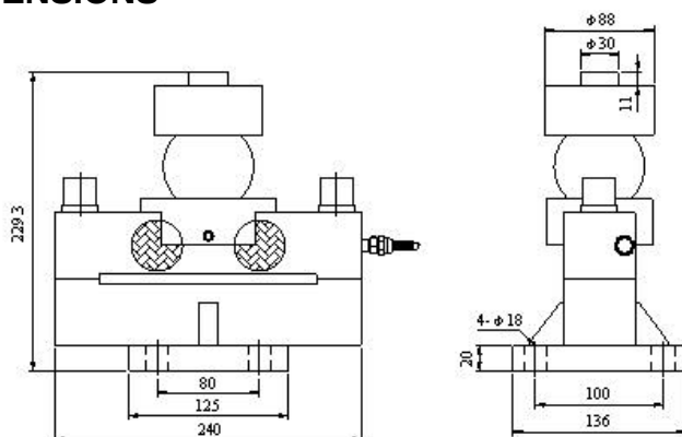
右视 (Right View)
